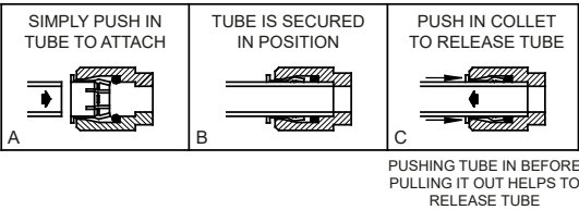
Fig 6: Poly Tube Quick Connect Fitting
