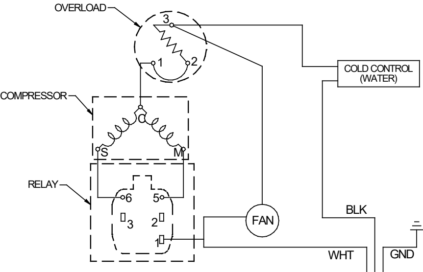
Fig 8: 115V Wiring Diagram
