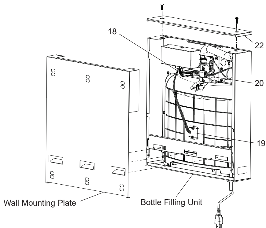
Fig 5: Front View with Aerator
