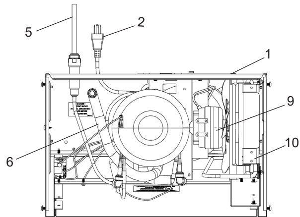
Fig 1: Cooler Top View (EZ8WS Shown)
