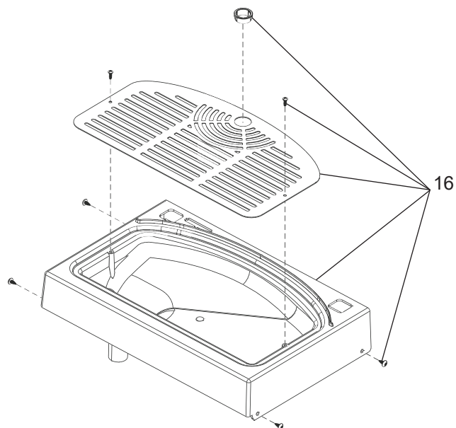
Fig 4: Basin Assembly Kit
