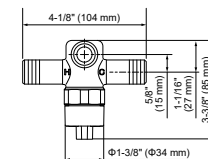
Thermostatic Mixing Valve (TLE05701U)
