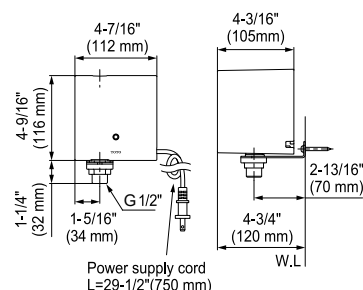
AC Controller
