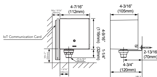
ECOPOWER Controller
