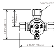
Hot/Cold Mixing Tee (TLM10)
