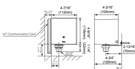
ECOPOWER Controller
