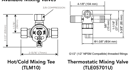
Available Mixing Valves
