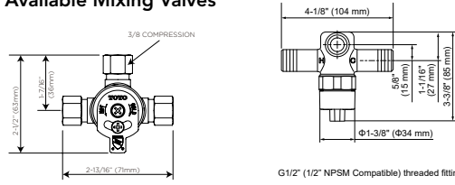
Hot/Cold Mixing Tee (TLM10)
